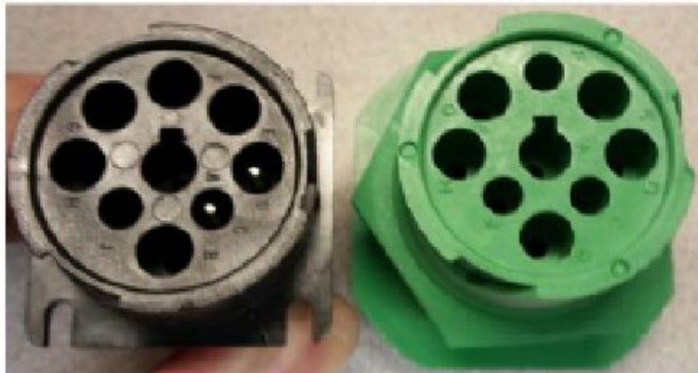
250k Connector
